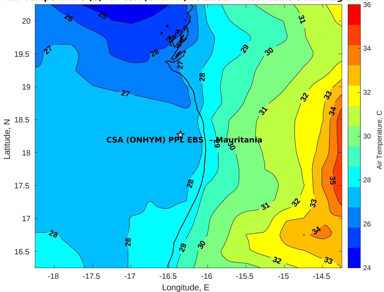
Air Temperature (C) for CSA (ONHYM) PPL EBS - Mauritania at 11-Aug-2025
