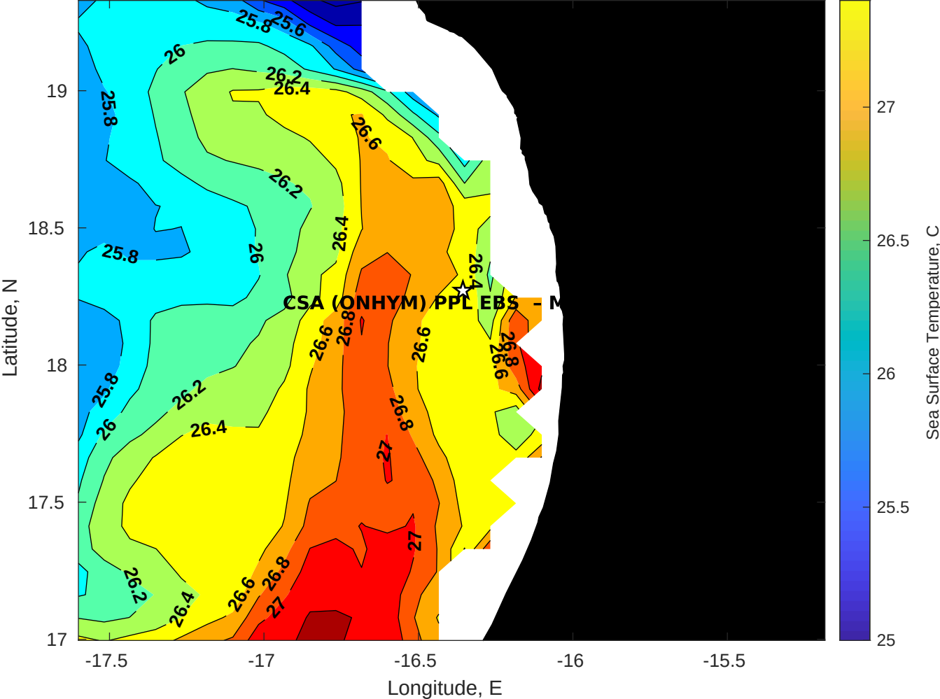
SST for CSA (ONHYM) PPL EBS - Mauritania at 10-Aug-2025 00:00:00
