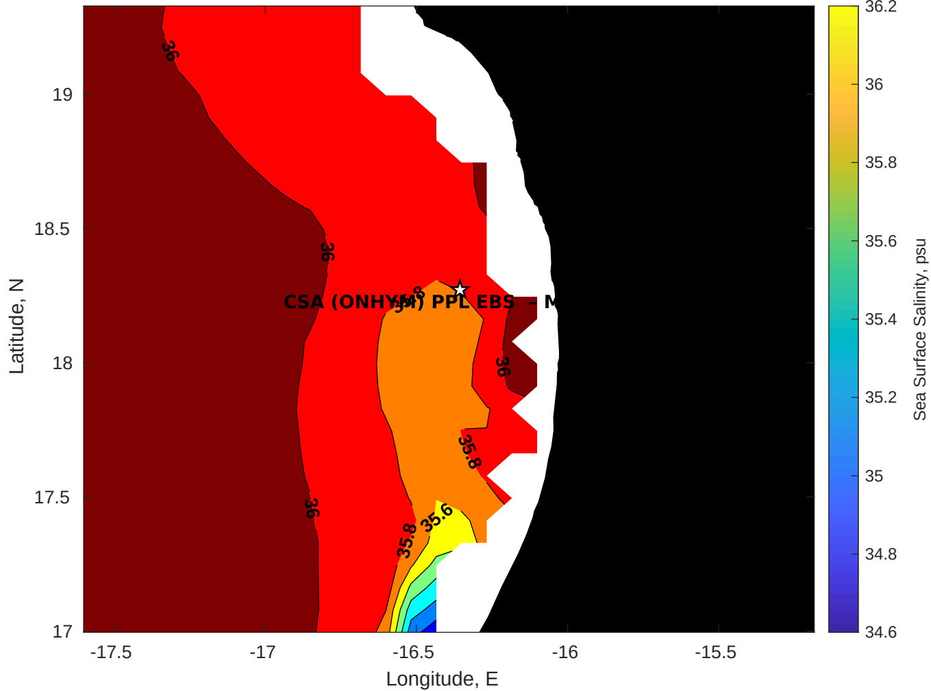
Surface Salinity for CSA (ONHYM) PPL EBS - Mauritania at 10-Aug-2025 00:00:00
