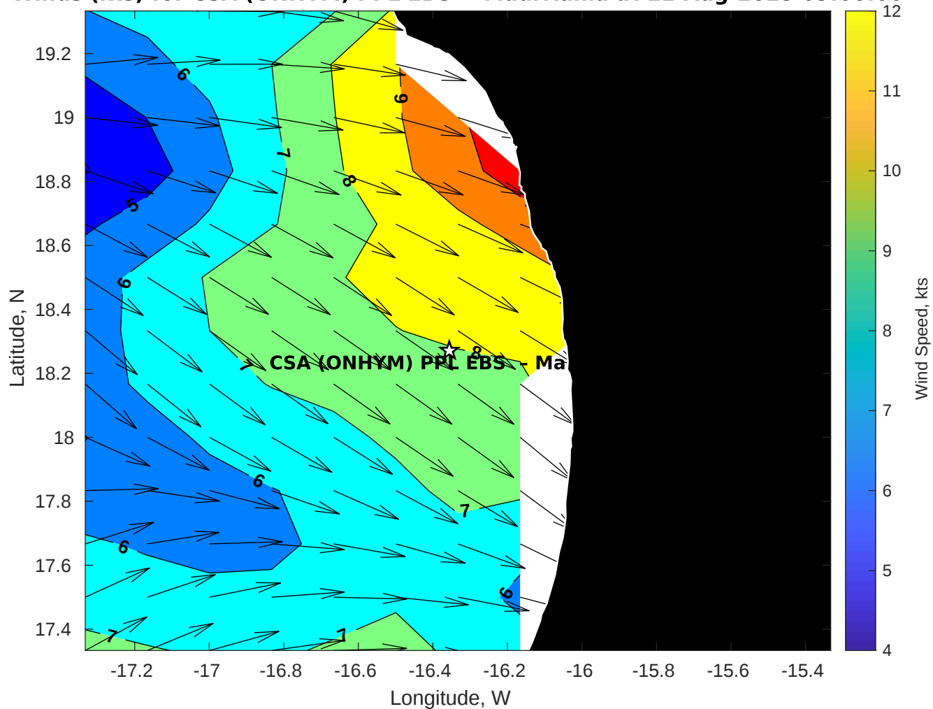
Winds (kts) for CSA (ONHYM) PPL EBS - Mauritania at 11-Aug-2025 09:00:00
