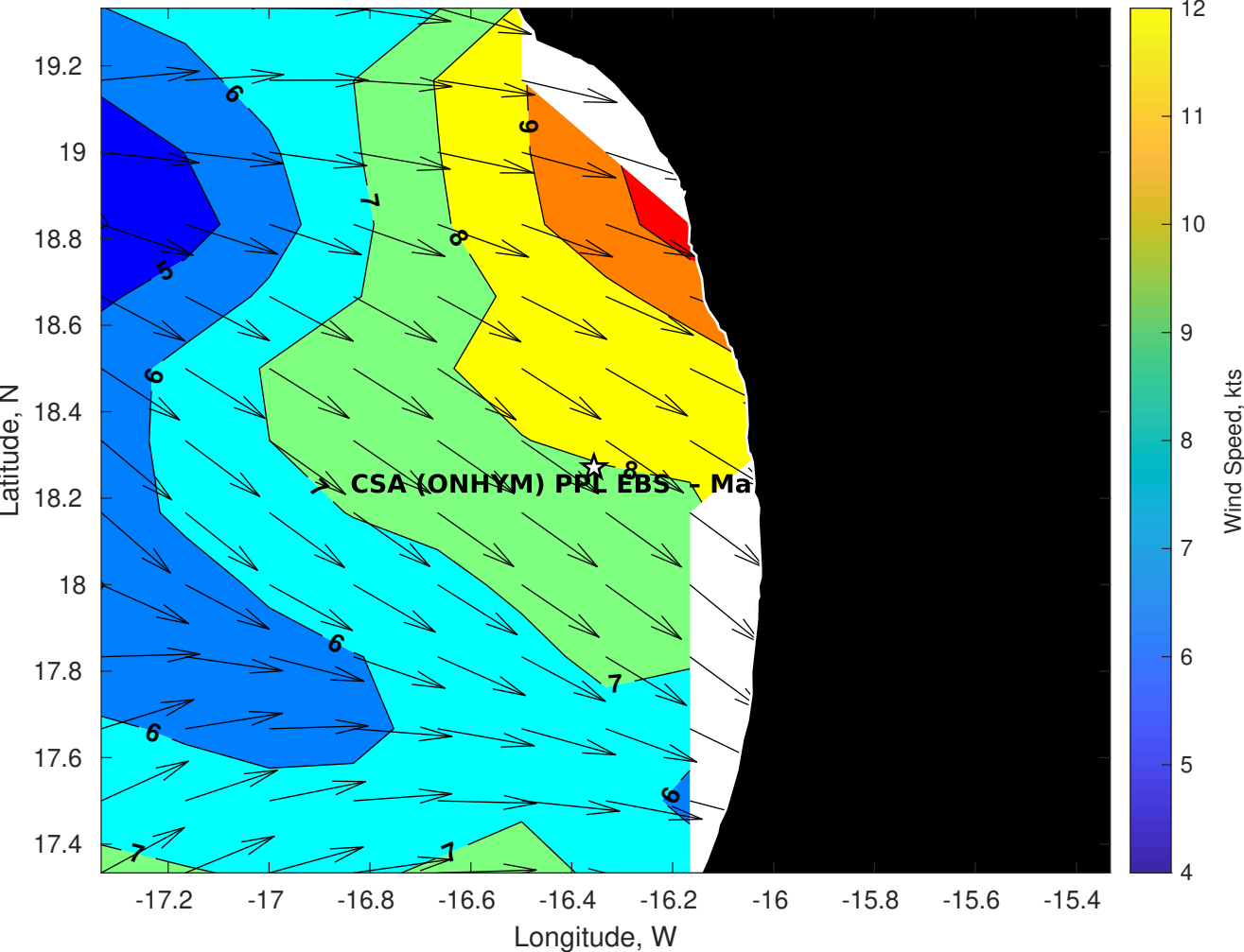
Winds (kts) for CSA (ONHYM) PPL EBS - Mauritania at 11-Aug-2025 09:00:00
