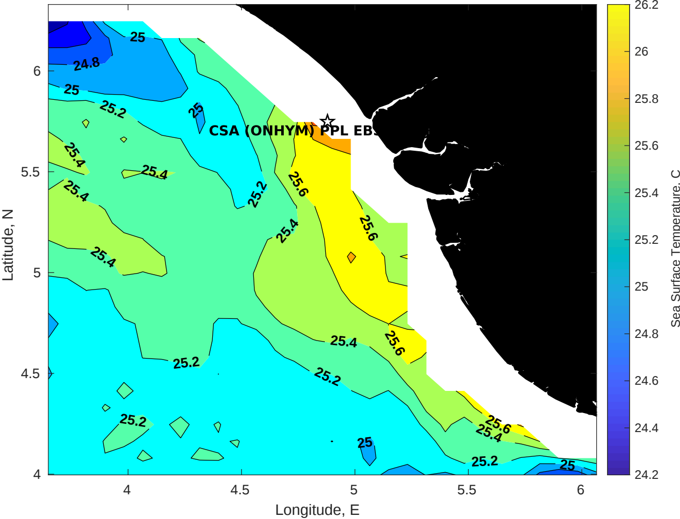
SST for CSA (ONHYM) PPL EBS - Nigeria at 10-Aug-2025 00:00:00
