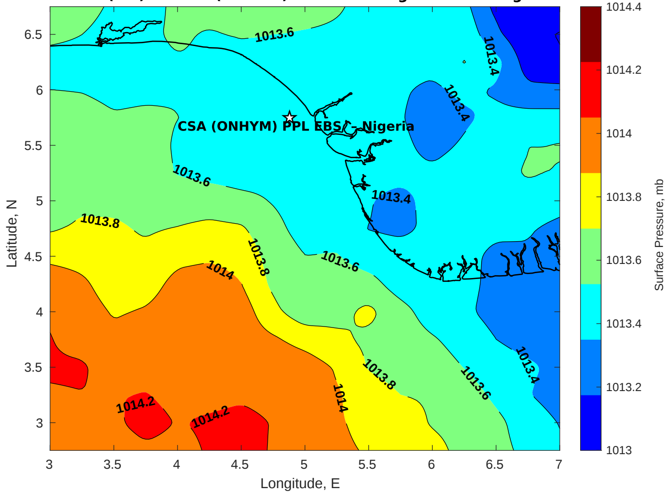
Surface Pressure (mb) for CSA (ONHYM) PPL EBS - Nigeria at 12-Aug-2025 00:00:00
