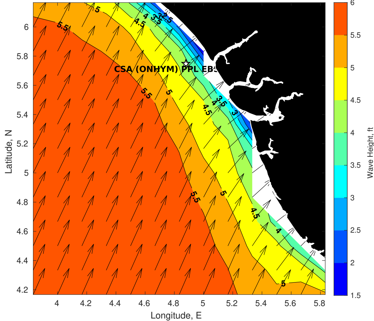
Wave Height (ft) for CSA (ONHYM) PPL EBS - Nigeria at 11-Aug-2025 09:00:00
