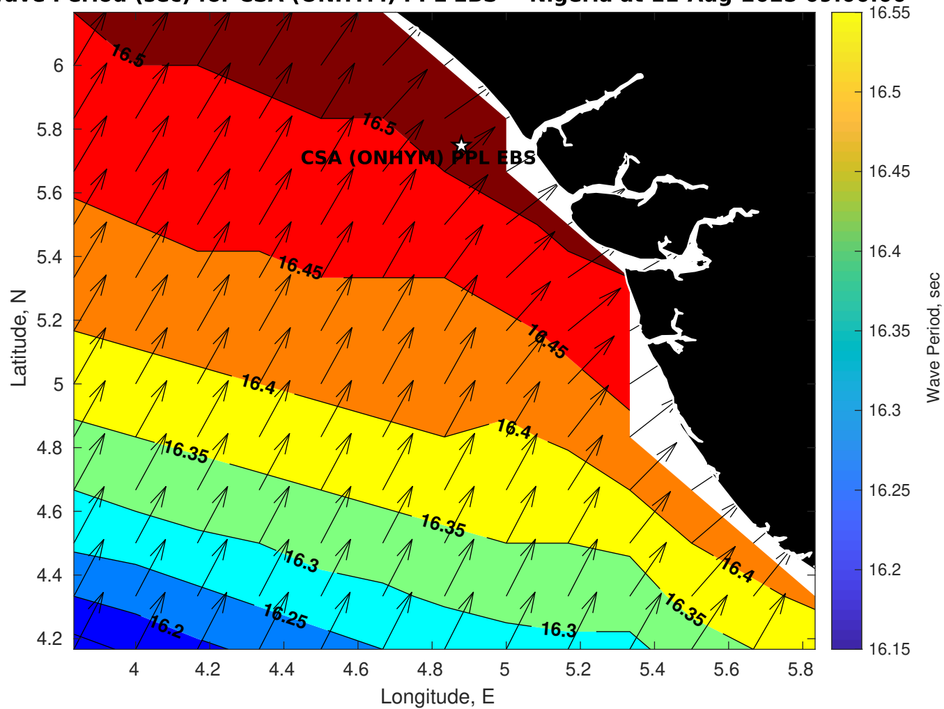
Wave Period (sec) for CSA (ONHYM) PPL EBS - Nigeria at 11-Aug-2025 09:00:00
