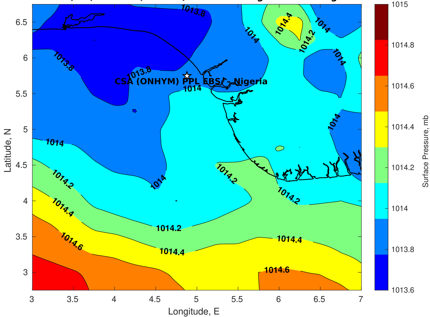
Surface Pressure (mb) for CSA (ONHYM) PPL EBS - Nigeria at 13-Aug-2025 00:00:00
