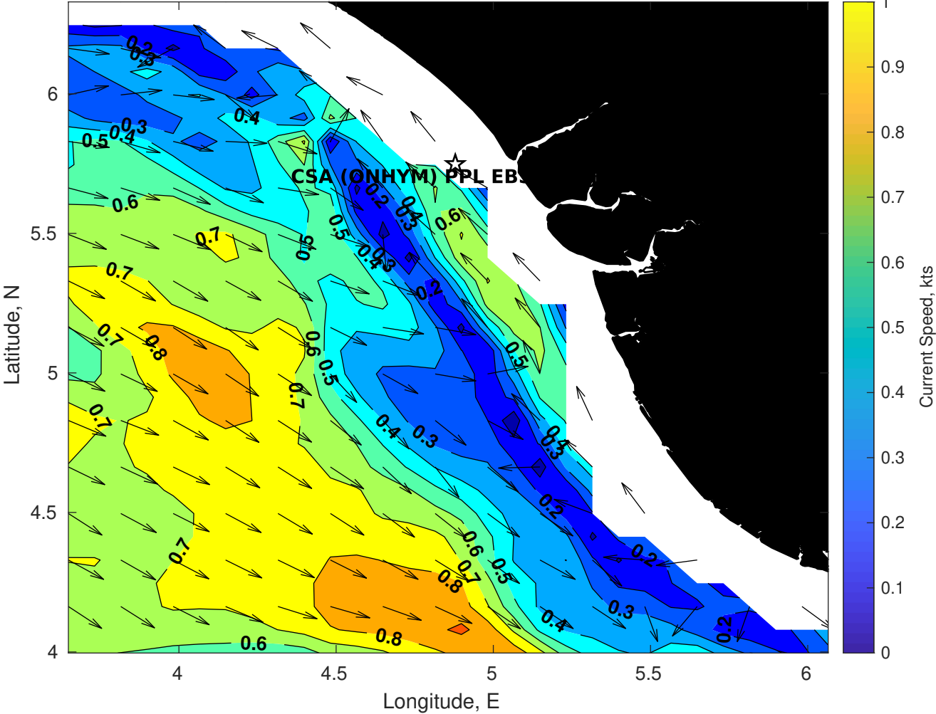
Surface Currents for CSA (ONHYM) PPL EBS - Nigeria at 10-Aug-2025 00:00:00
