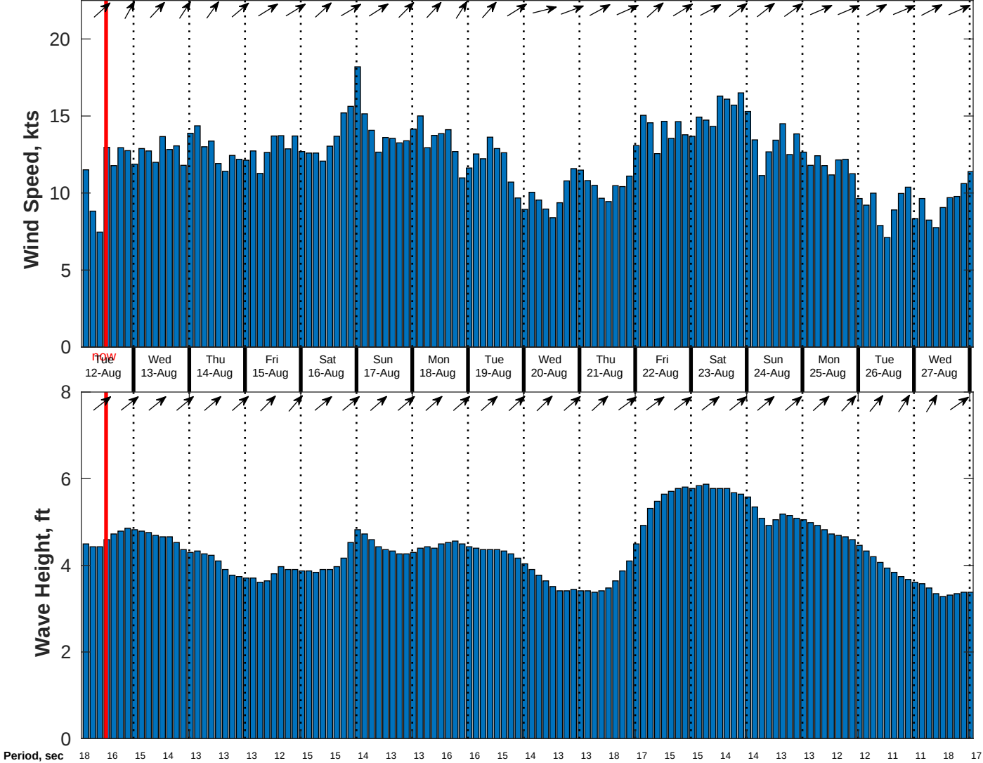
Wind & Wave Forecast for CSA (ONHYM) PPL EBS - Nigeria from 11-Aug-2025 02:00:00 to 27-Aug-2025 02:00:00
