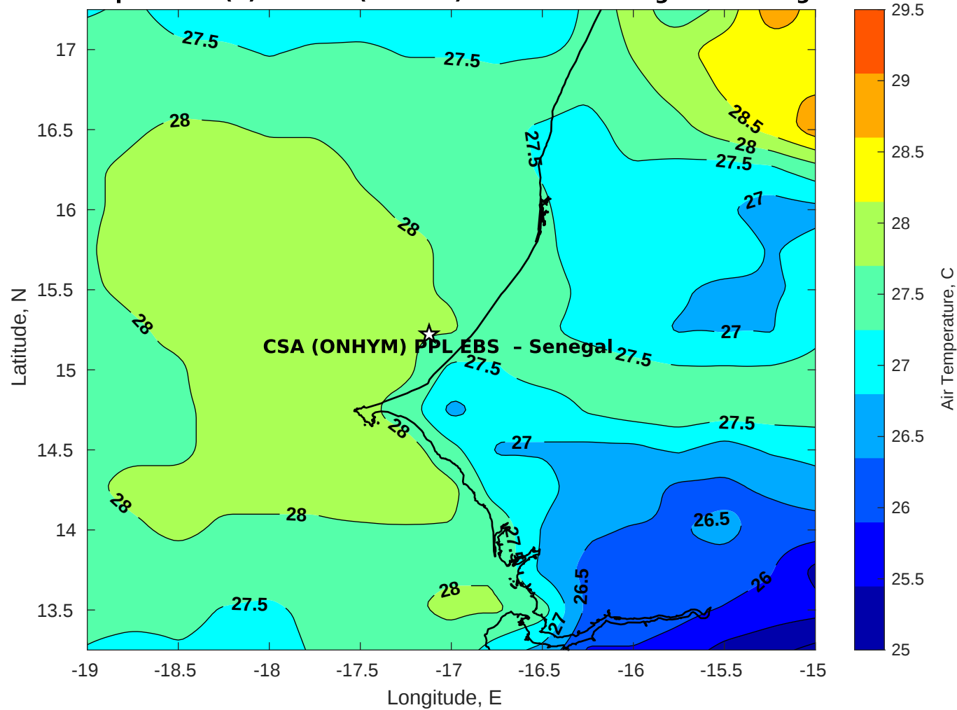
Air Temperature (C) for CSA (ONHYM) PPL EBS - Senegal at 11-Aug-2025
