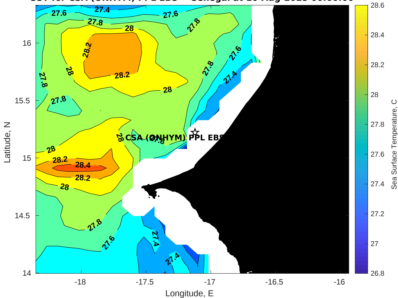
SST for CSA (ONHYM) PPL EBS - Senegal at 10-Aug-2025 00:00:00
