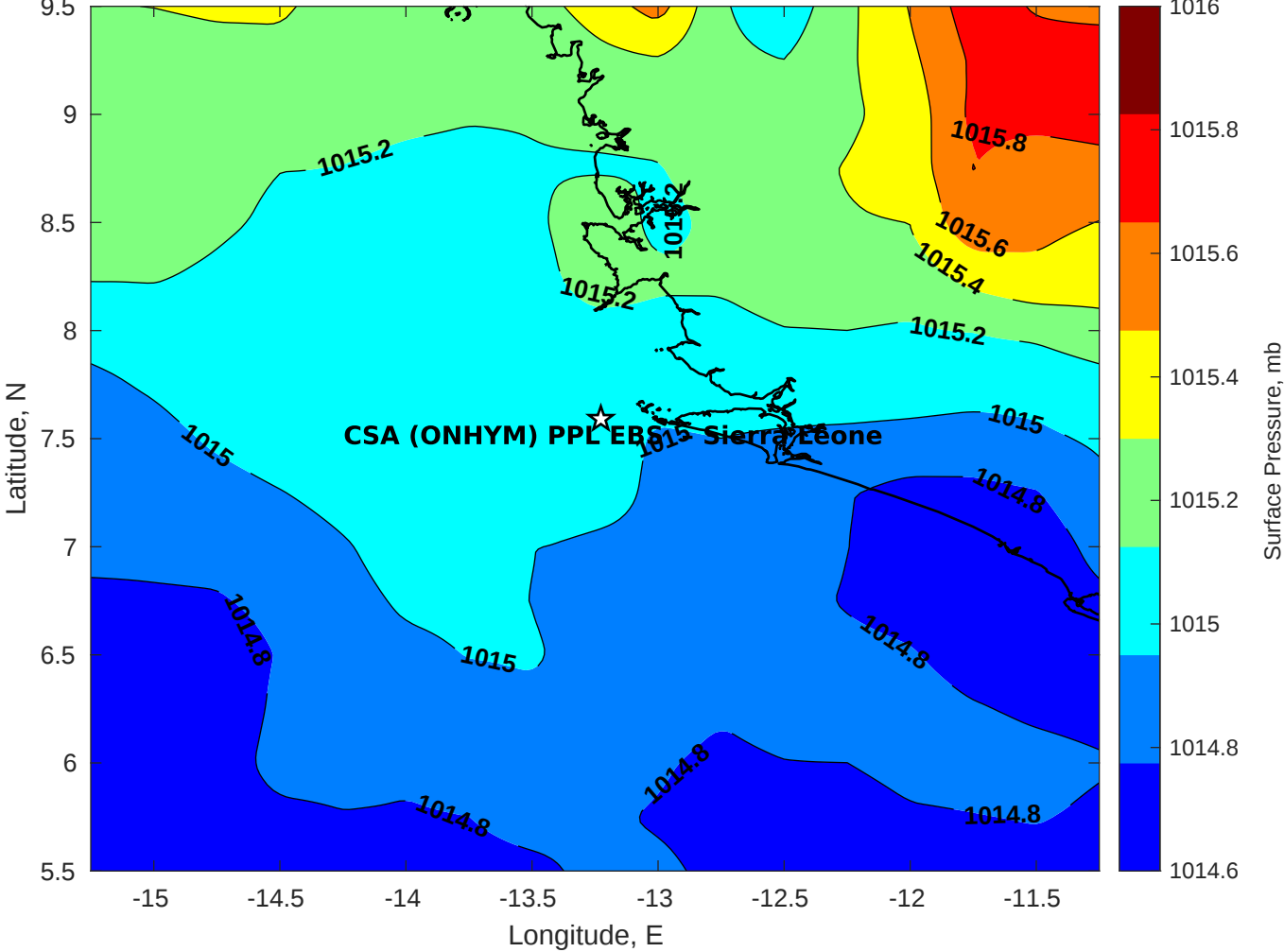
Surface Pressure (mb) for CSA (ONHYM) PPL EBS - Sierra Leone at 11-Aug-2025 00:00:00
