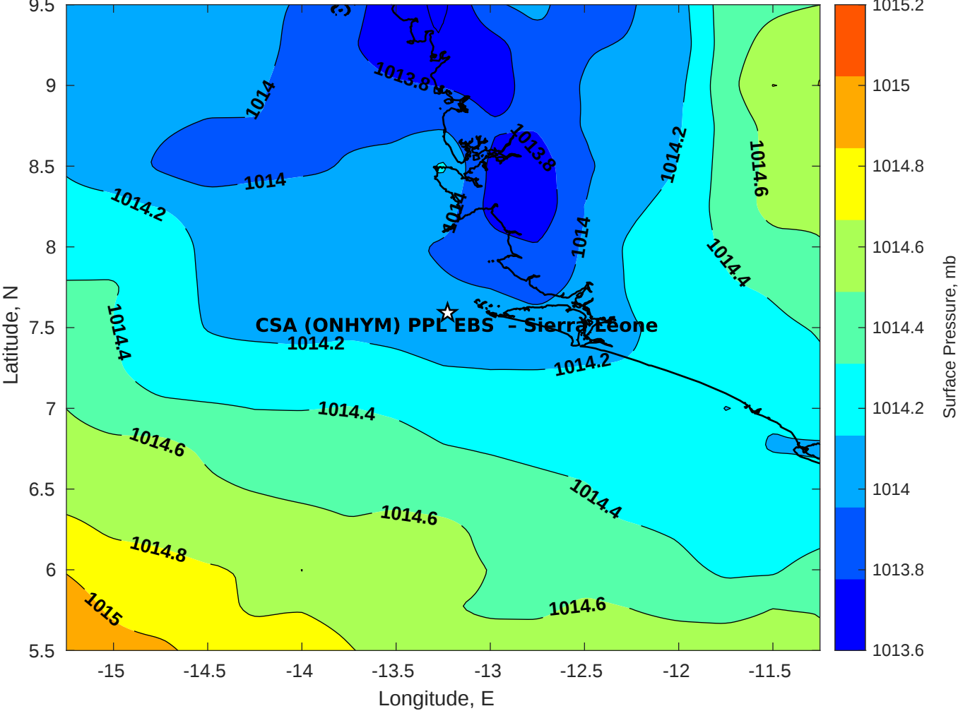
Surface Pressure (mb) for CSA (ONHYM) PPL EBS - Sierra Leone at 12-Aug-2025 00:00:00
