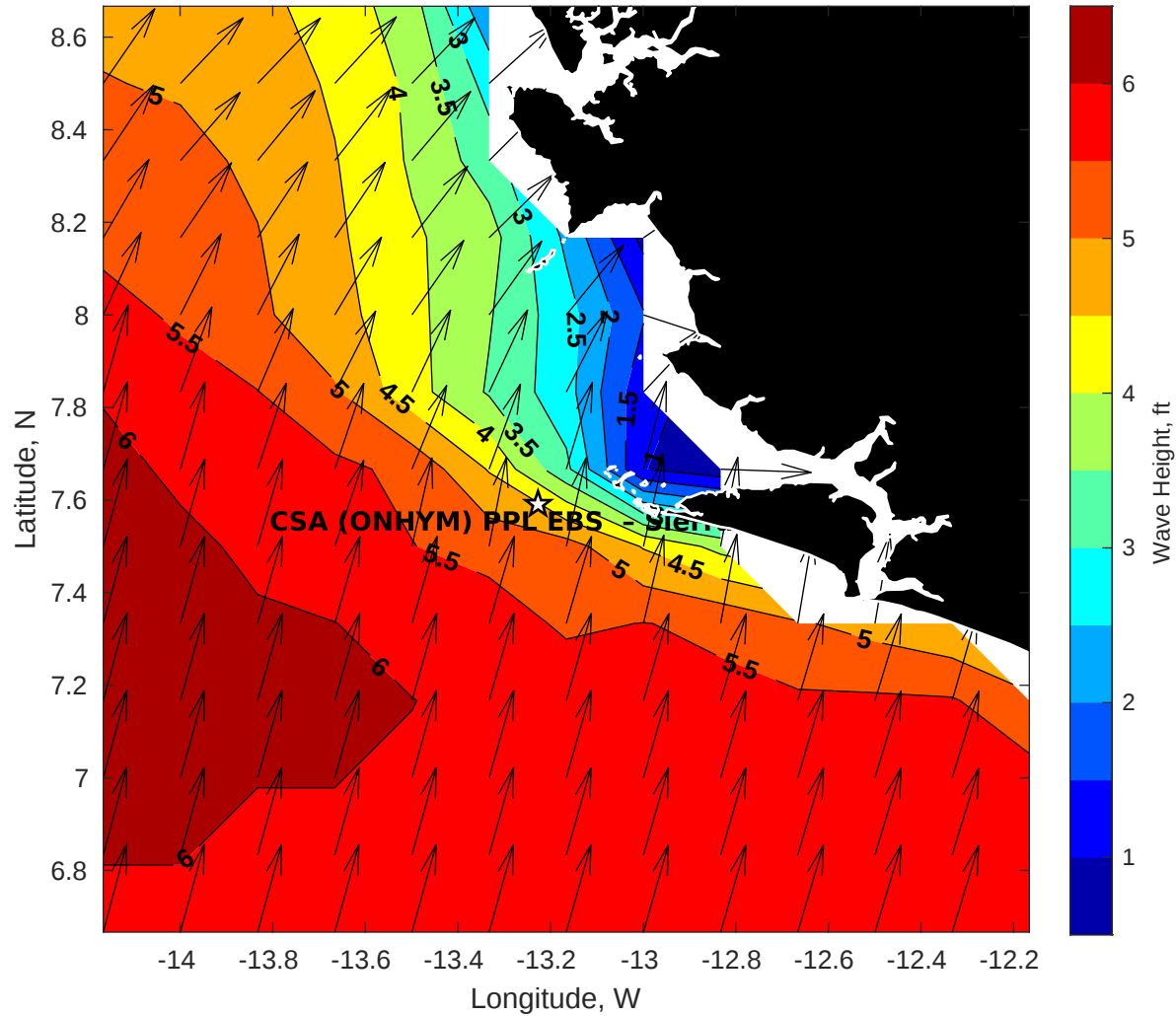
Wave Height (ft) for CSA (ONHYM) PPL EBS - Sierra Leone at 11-Aug-2025 09:00:00
