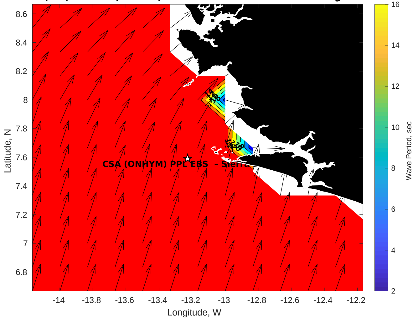
Wave Period (sec) for CSA (ONHYM) PPL EBS - Sierra Leone at 11-Aug-2025 09:00:00
