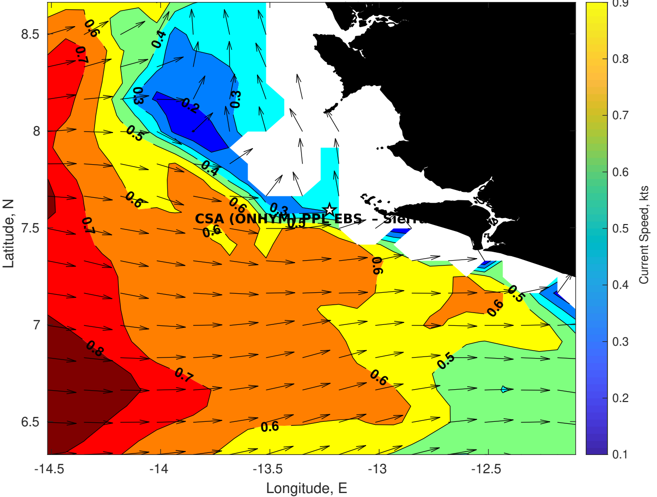
Surface Currents for CSA (ONHYM) PPL EBS - Sierra Leone at 10-Aug-2025 00:00:00
