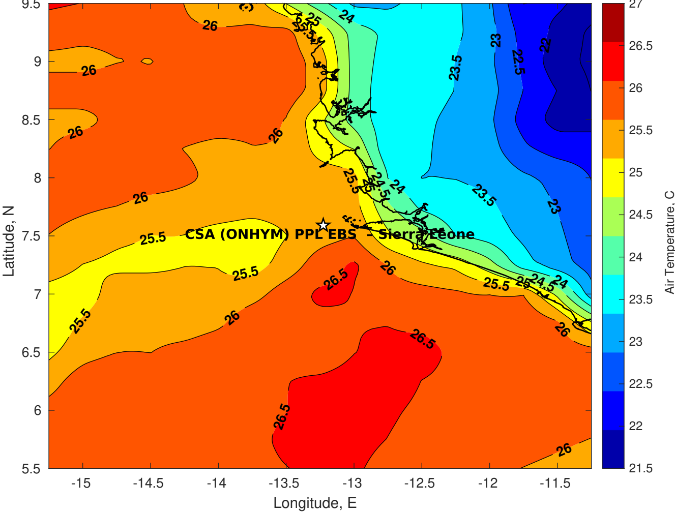
Air Temperature (C) for CSA (ONHYM) PPL EBS - Sierra Leone at 11-Aug-2025
