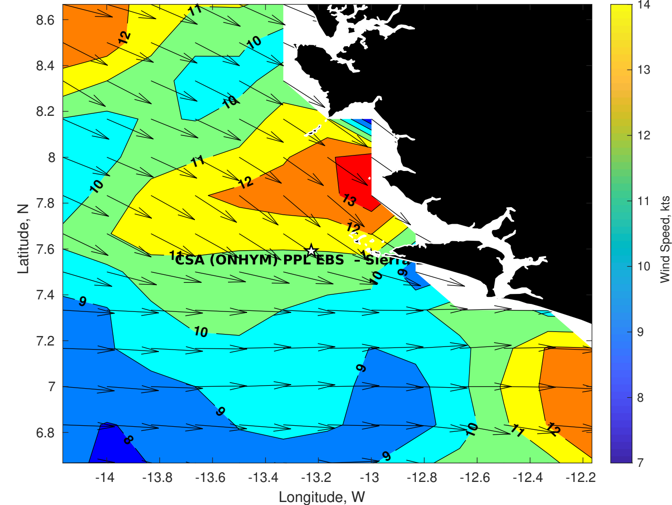
Winds (kts) for CSA (ONHYM) PPL EBS - Sierra Leone at 11-Aug-2025 09:00:00
