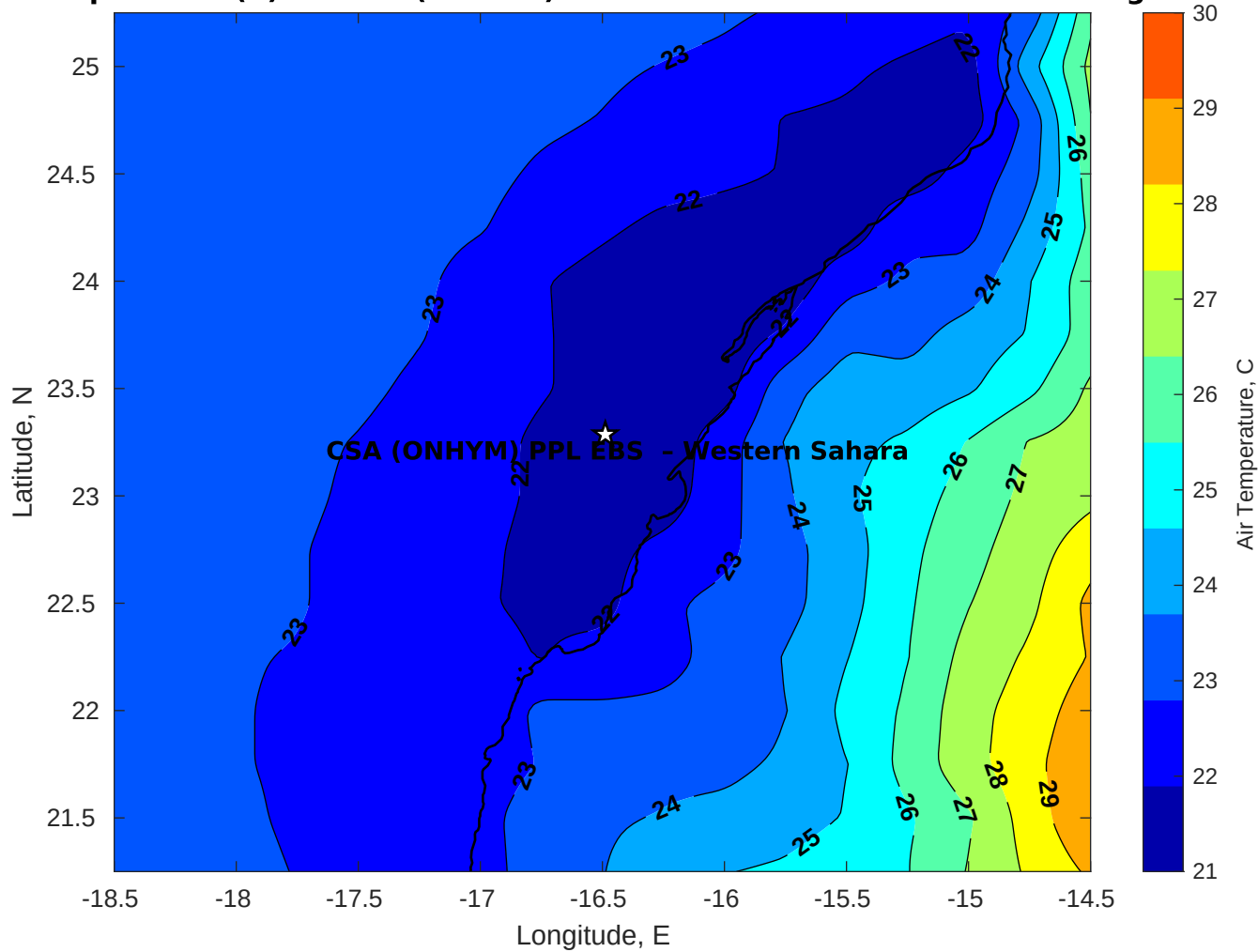
Air Temperature (C) for CSA (ONHYM) PPL EBS - Western Sahara at 11-Aug-2025
