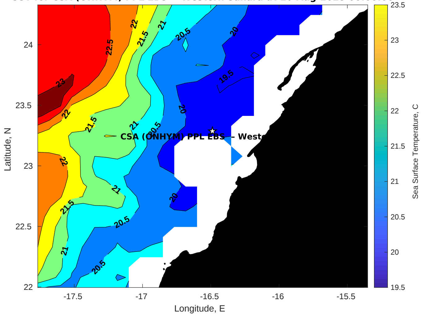
SST for CSA (ONHYM) PPL EBS - Western Sahara at 10-Aug-2025 00:00:00
