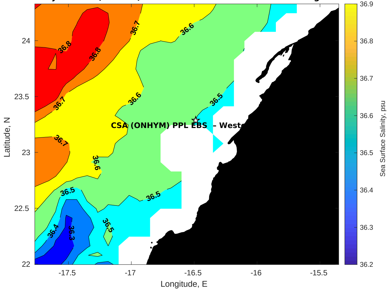
Surface Salinity for CSA (ONHYM) PPL EBS - Western Sahara at 10-Aug-2025 00:00:00
