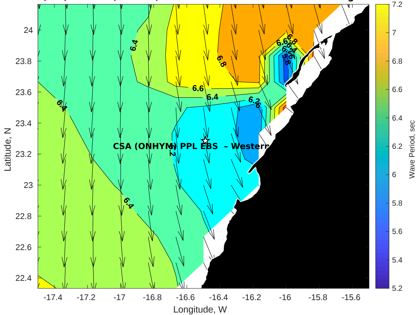
Wave Period (sec) for CSA (ONHYM) PPL EBS - Western Sahara at 11-Aug-2025 09:00:00
