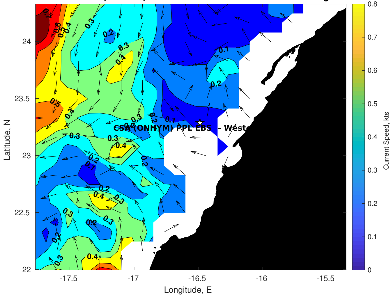
Surface Currents for CSA (ONHYM) PPL EBS - Western Sahara at 10-Aug-2025 00:00:00
