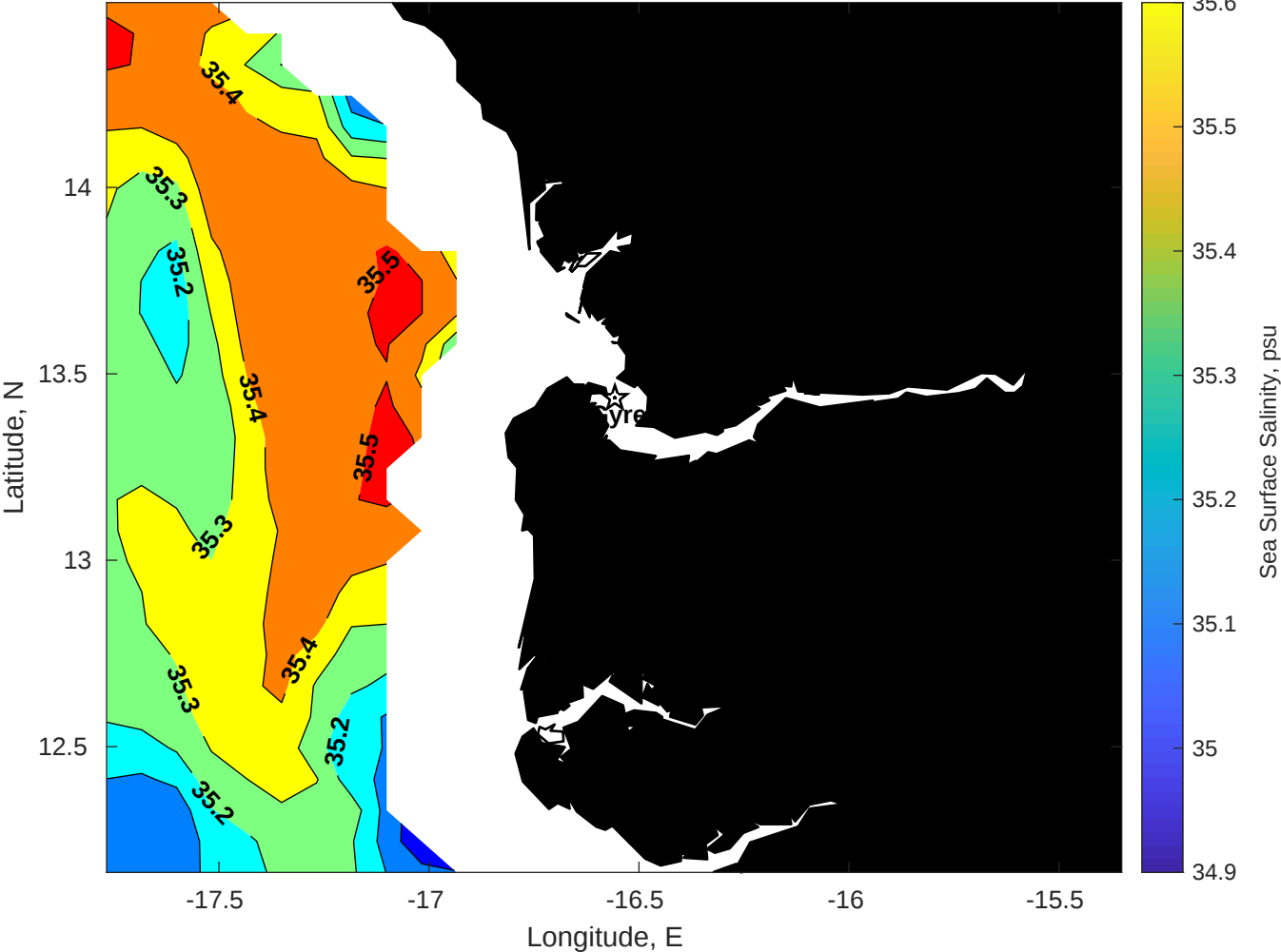
Surface Salinity for Gyre at 10-Aug-2025 00:00:00
