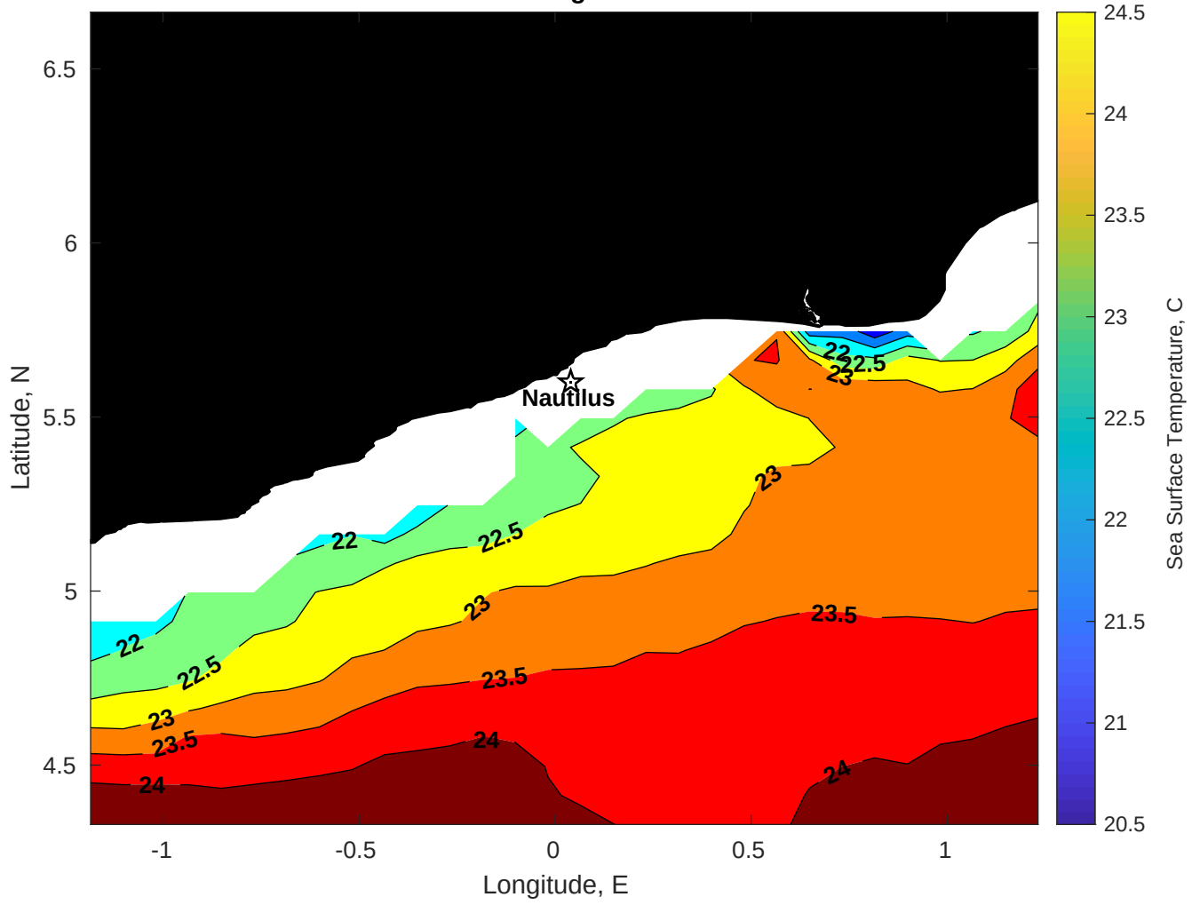
SST for Nautilus at 10-Aug-2025 00:00:00
