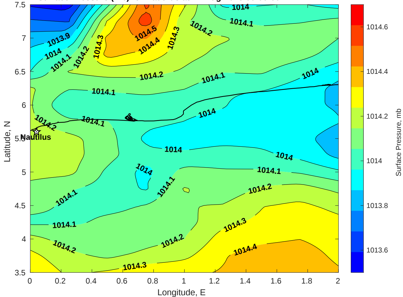
Surface Pressure (mb) for Nautilus at 12-Aug-2025 00:00:00
