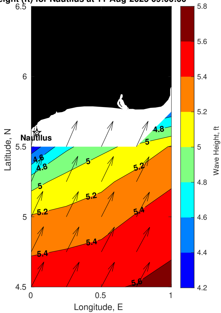
Wave Height (ft) for Nautilus at 11-Aug-2025 09:00:00
