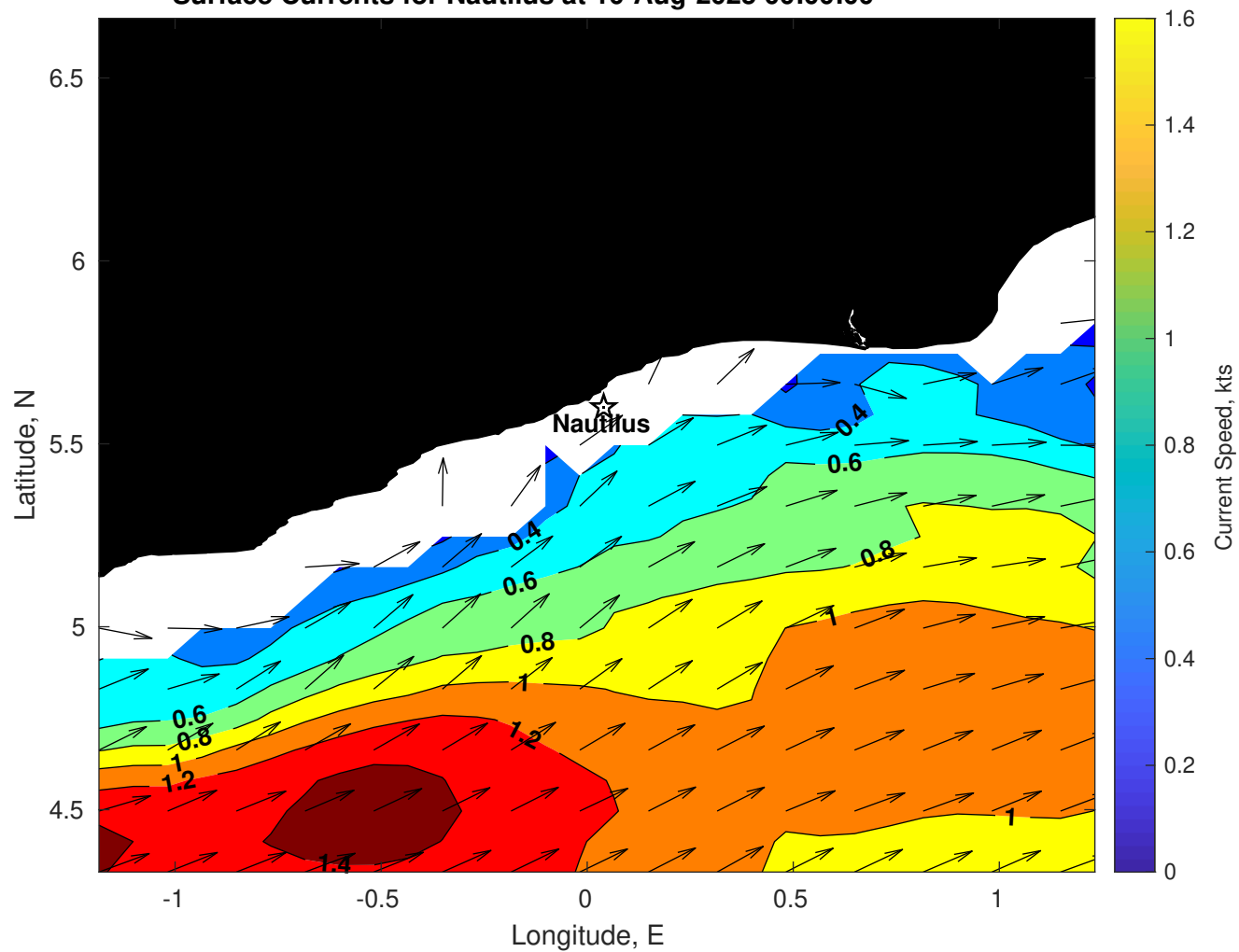
Surface Currents for Nautilus at 10-Aug-2025 00:00:00
