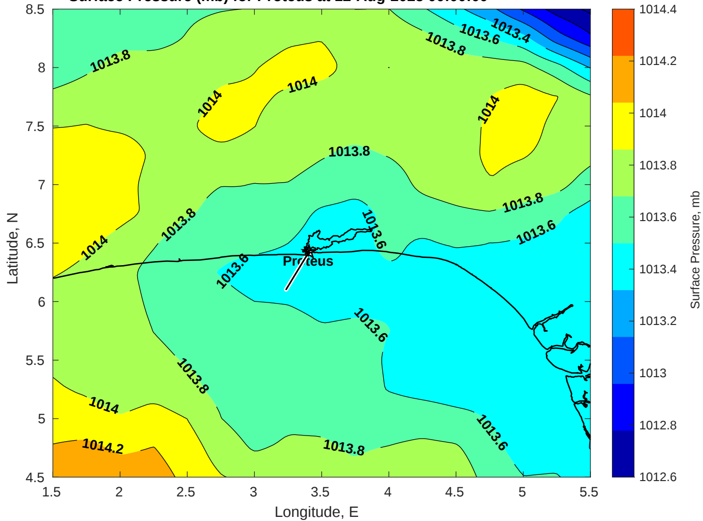
Surface Pressure (mb) for Proteus at 12-Aug-2025 00:00:00
