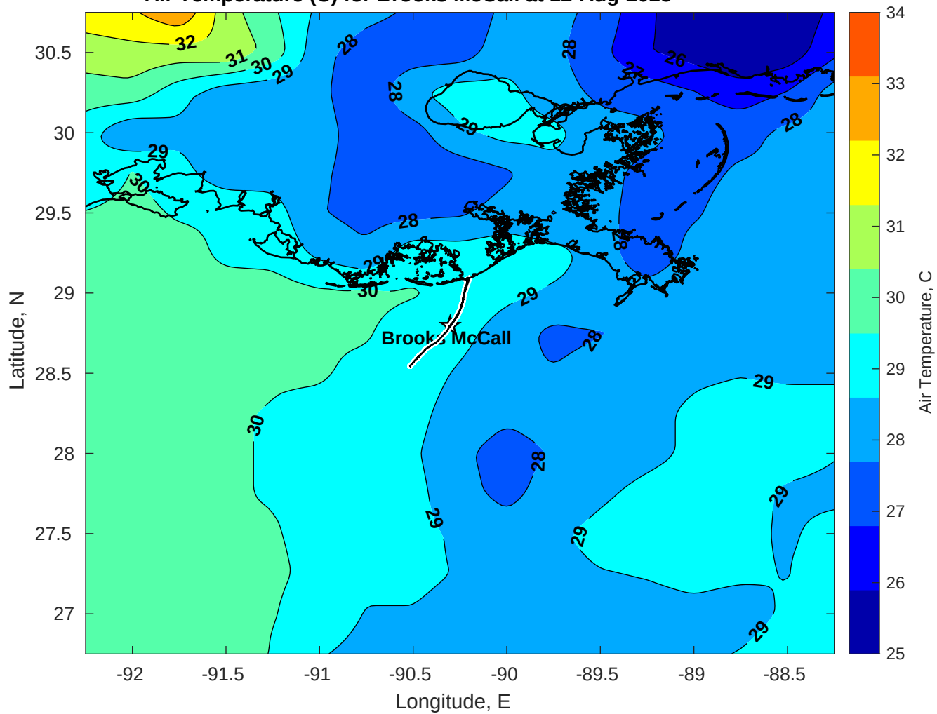
Air Temperature (C) for Brooks McCall at 12-Aug-2025
