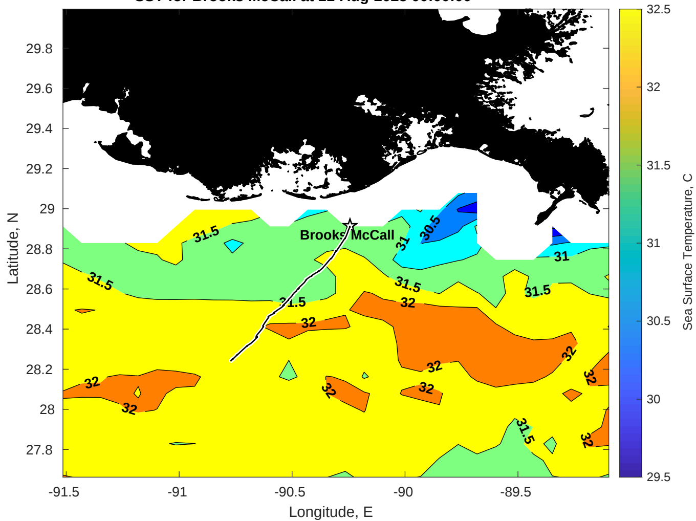
SST for Brooks McCall at 11-Aug-2025 00:00:00
