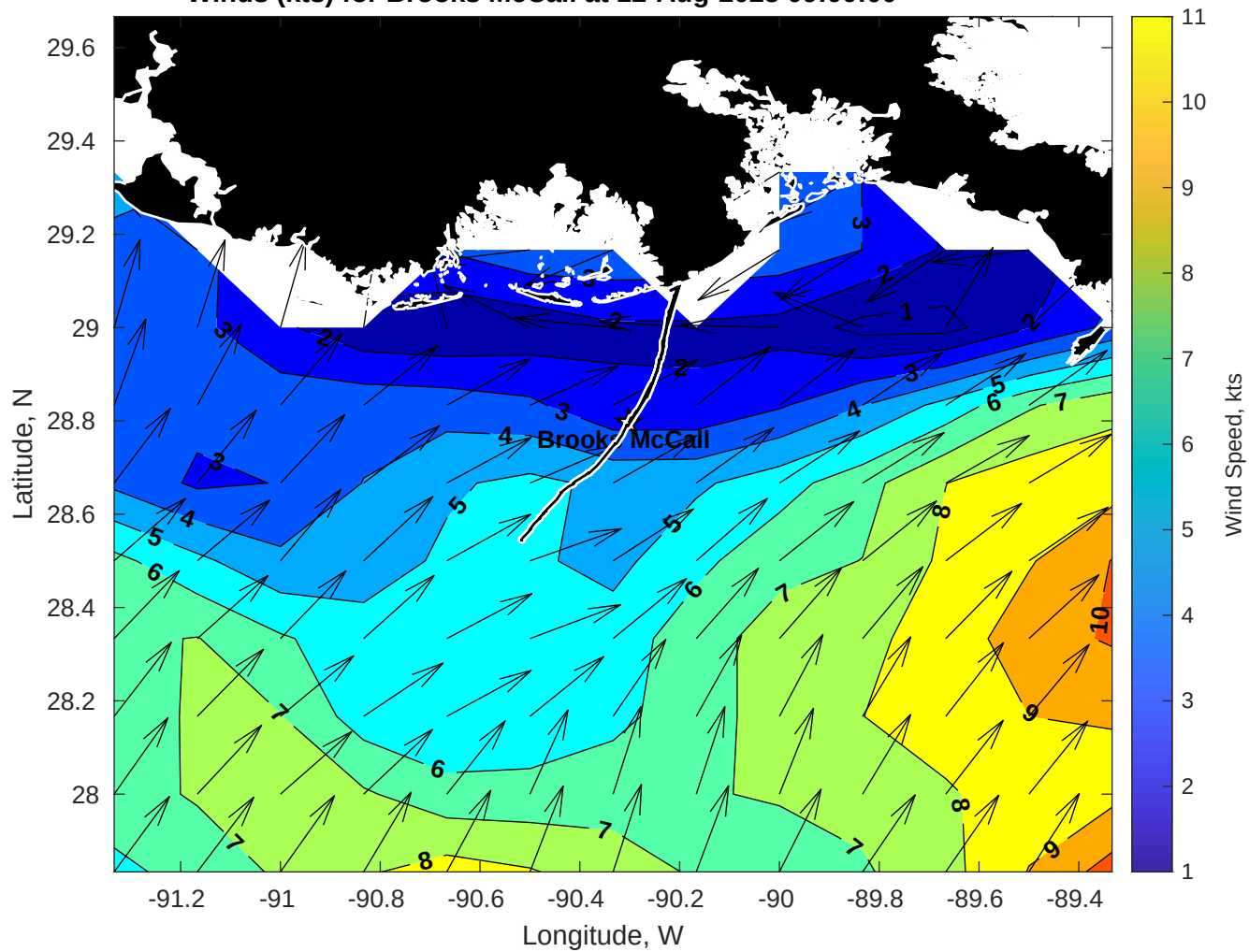
Winds (kts) for Brooks McCall at 12-Aug-2025 09:00:00
