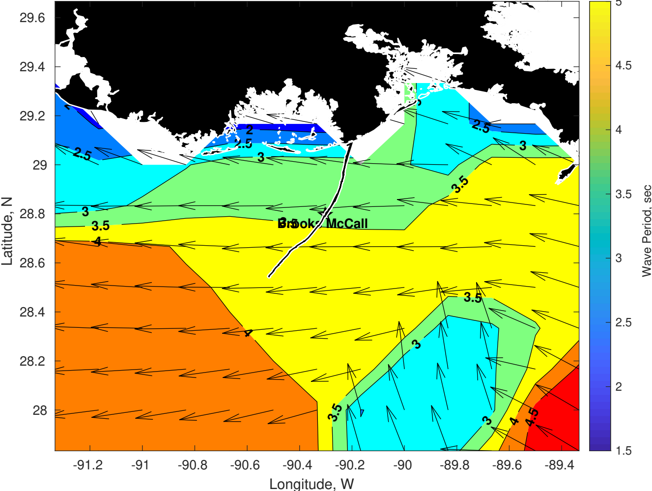
Wave Period (sec) for Brooks McCall at 12-Aug-2025 09:00:00
