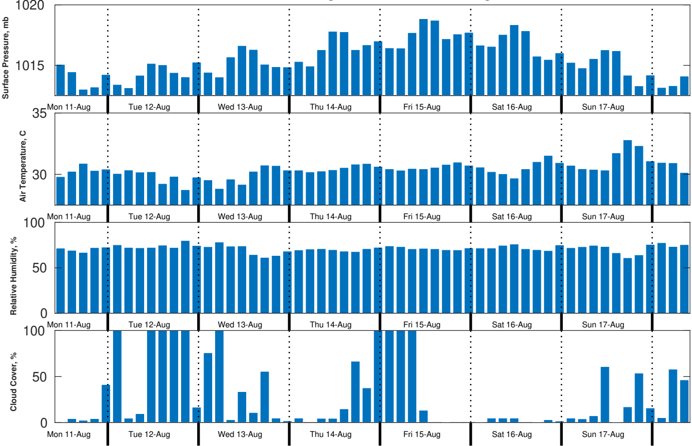
Met Forecast for Brooks McCall from 11-Aug-2025 12:00:00 to 18-Aug-2025 12:00:00
