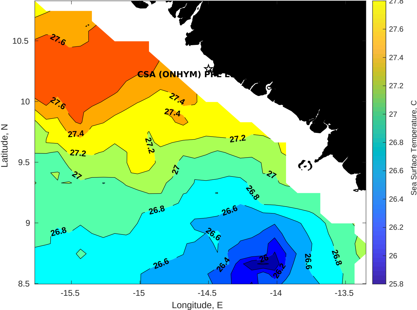
SST for CSA (ONHYM) PPL EBS - Guinea at 11-Aug-2025 00:00:00
