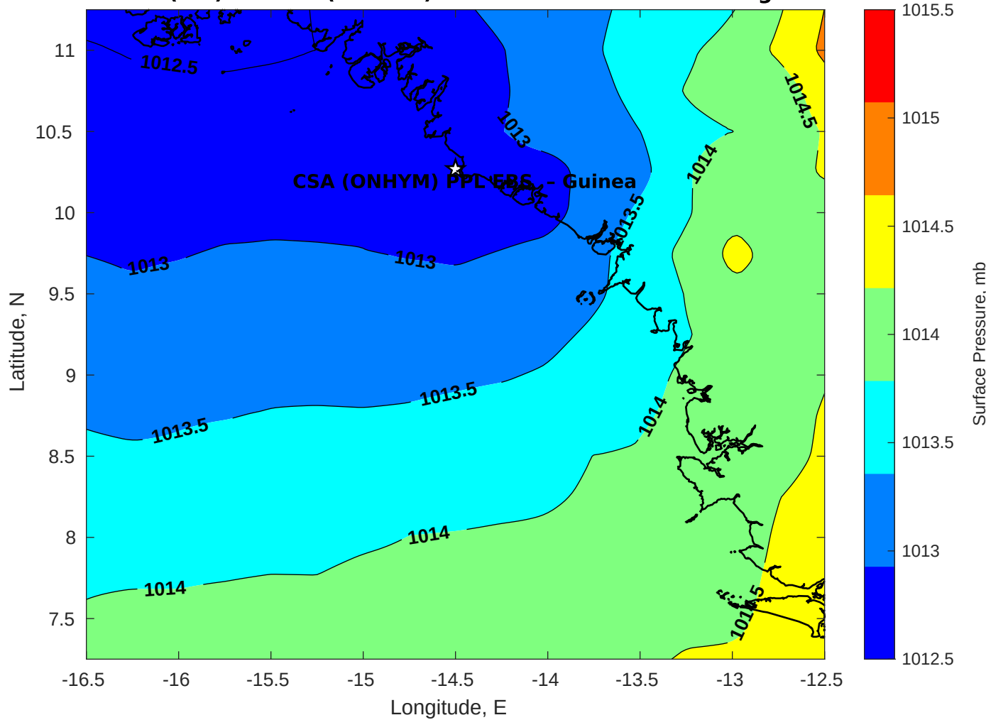
Surface Pressure (mb) for CSA (ONHYM) PPL EBS - Guinea at 13-Aug-2025 00:00:00
