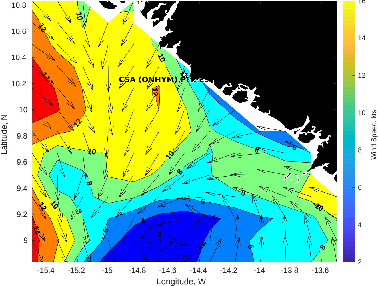
Winds (kts) for CSA (ONHYM) PPL EBS - Guinea at 12-Aug-2025 09:00:00
