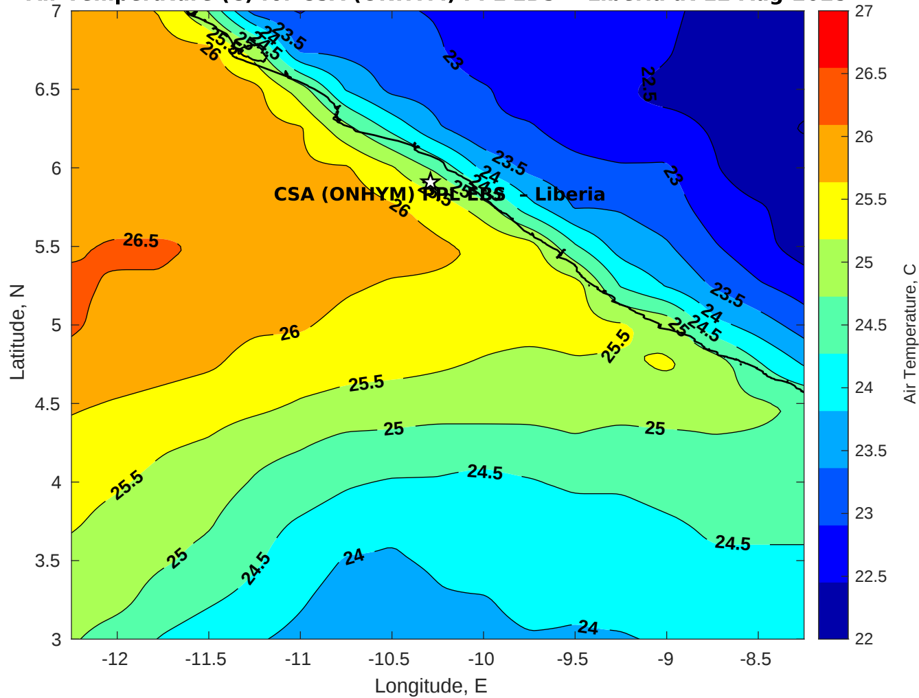
Air Temperature (C) for CSA (ONHYM) PPL EBS - Liberia at 12-Aug-2025
