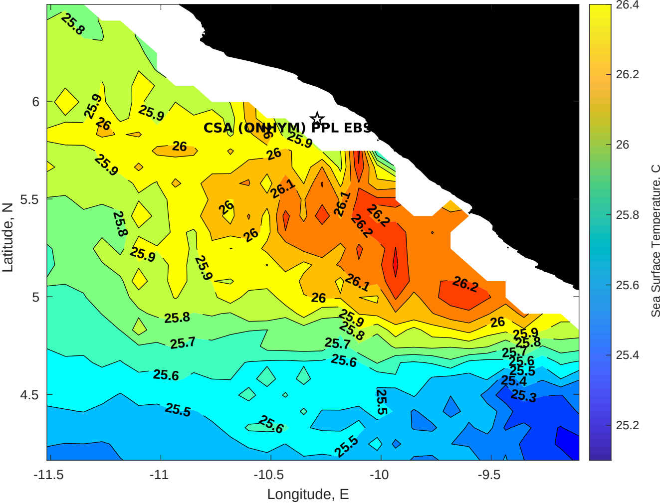
SST for CSA (ONHYM) PPL EBS - Liberia at 11-Aug-2025 00:00:00
