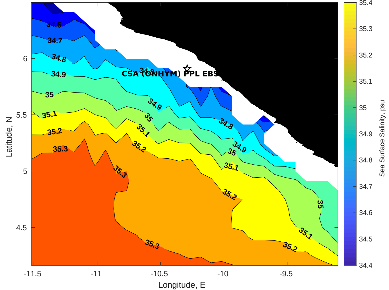
Surface Salinity for CSA (ONHYM) PPL EBS - Liberia at 11-Aug-2025 00:00:00
