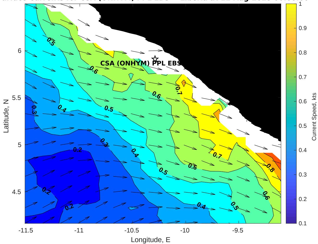
Surface Currents for CSA (ONHYM) PPL EBS - Liberia at 11-Aug-2025 00:00:00
