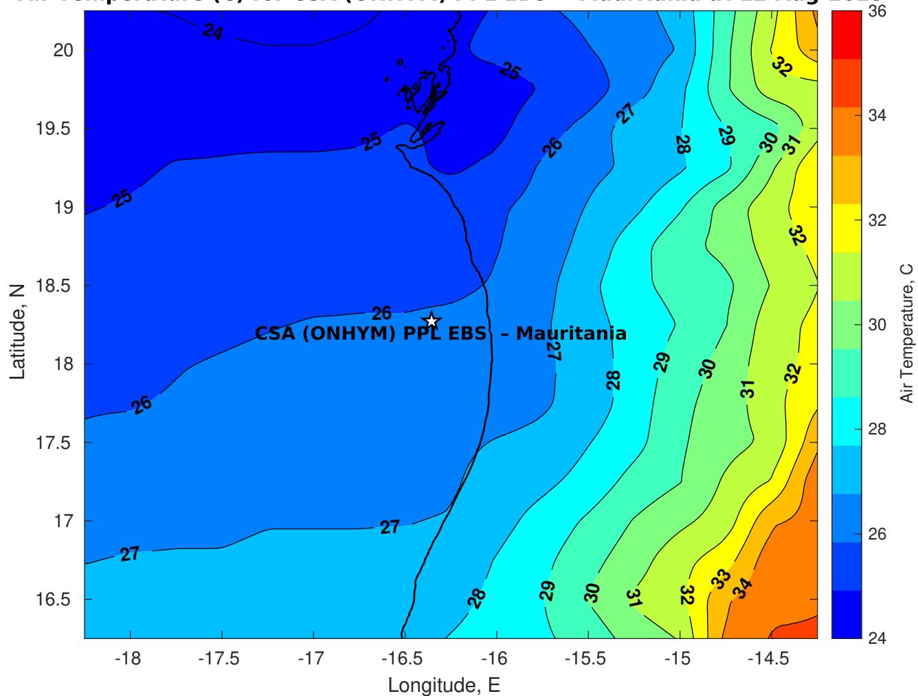
Air Temperature (C) for CSA (ONHYM) PPL EBS - Mauritania at 12-Aug-2025
