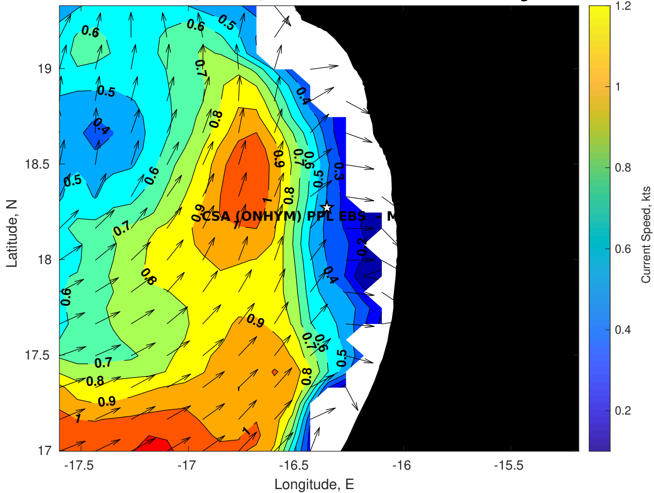
Surface Currents for CSA (ONHYM) PPL EBS - Mauritania at 11-Aug-2025 00:00:00
