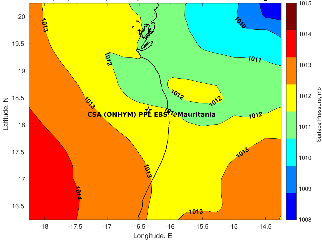
Surface Pressure (mb) for CSA (ONHYM) PPL EBS - Mauritania at 12-Aug-2025 00:00:00
