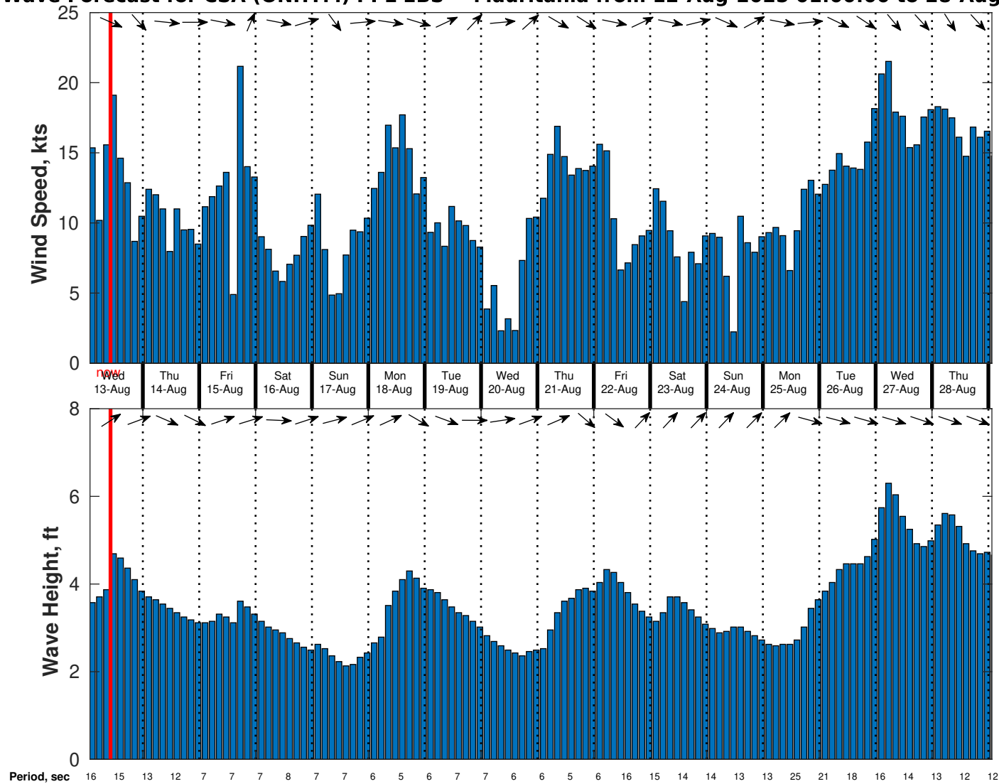
Wind & Wave Forecast for CSA (ONHYM) PPL EBS - Mauritania from 12-Aug-2025 01:00:00 to 28-Aug-2025 01:00:00
