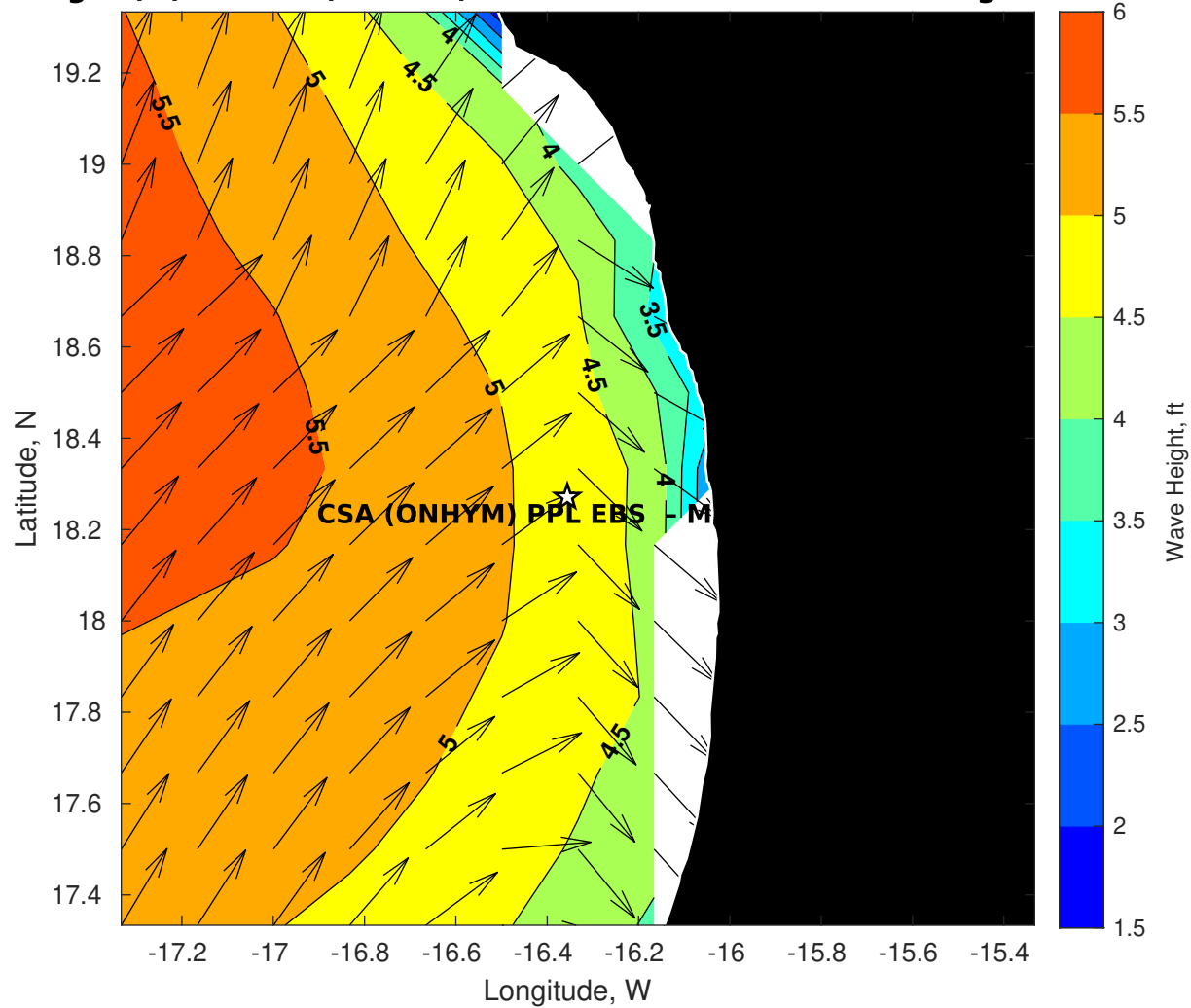
Wave Height (ft) for CSA (ONHYM) PPL EBS - Mauritania at 12-Aug-2025 09:00:00
