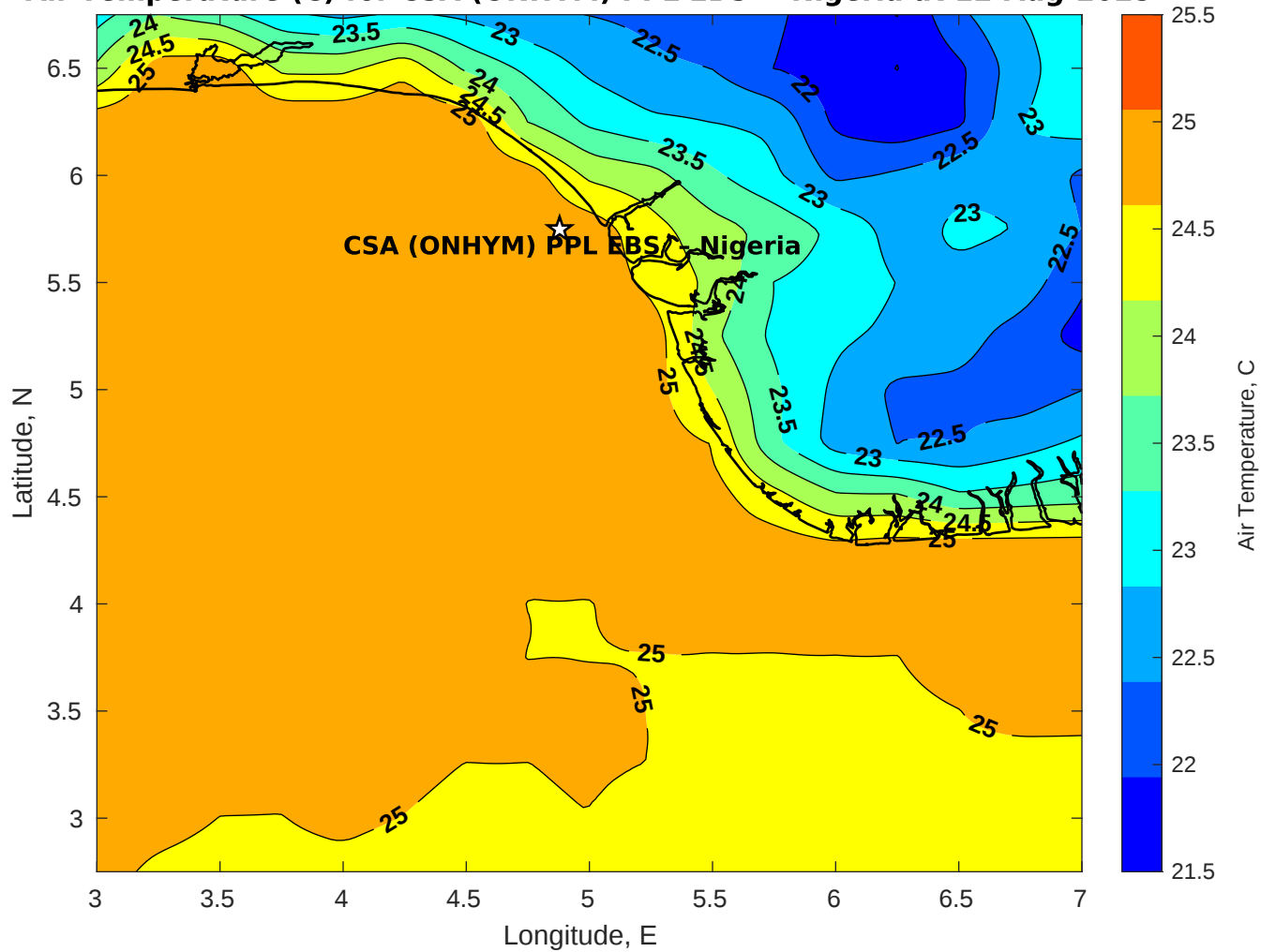
Air Temperature (C) for CSA (ONHYM) PPL EBS - Nigeria at 12-Aug-2025
