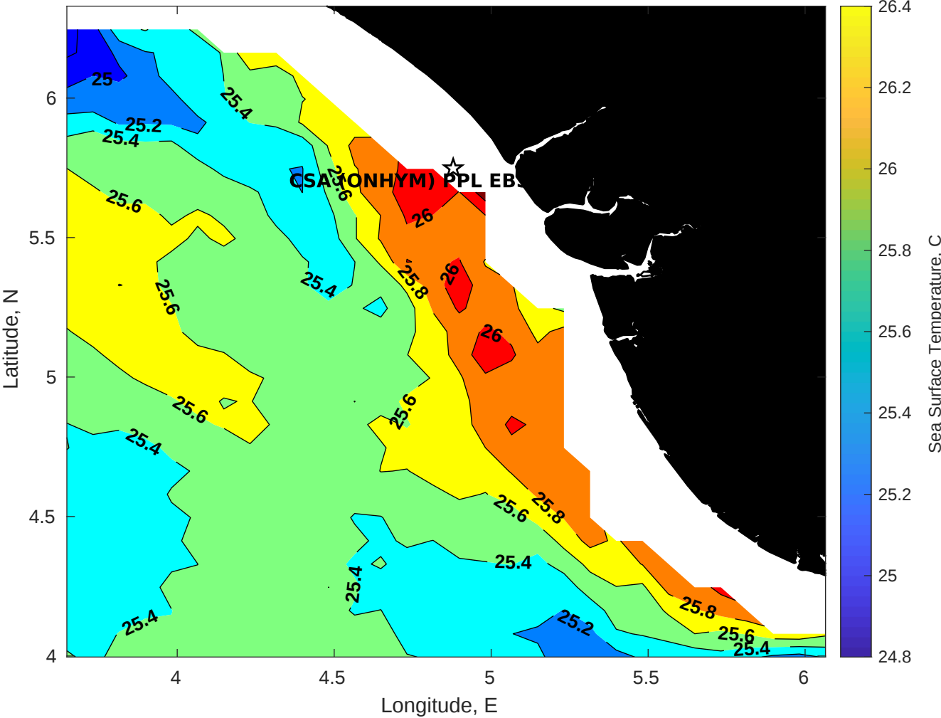
SST for CSA (ONHYM) PPL EBS - Nigeria at 11-Aug-2025 00:00:00
