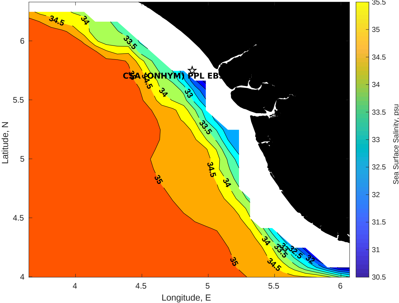
Surface Salinity for CSA (ONHYM) PPL EBS - Nigeria at 11-Aug-2025 00:00:00
