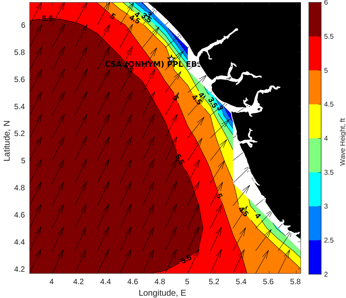
Wave Height (ft) for CSA (ONHYM) PPL EBS - Nigeria at 12-Aug-2025 09:00:00
