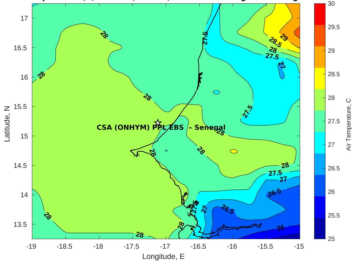
Air Temperature (C) for CSA (ONHYM) PPL EBS - Senegal at 12-Aug-2025
