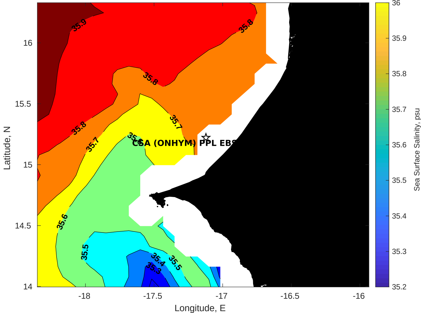
Surface Salinity for CSA (ONHYM) PPL EBS - Senegal at 11-Aug-2025 00:00:00
