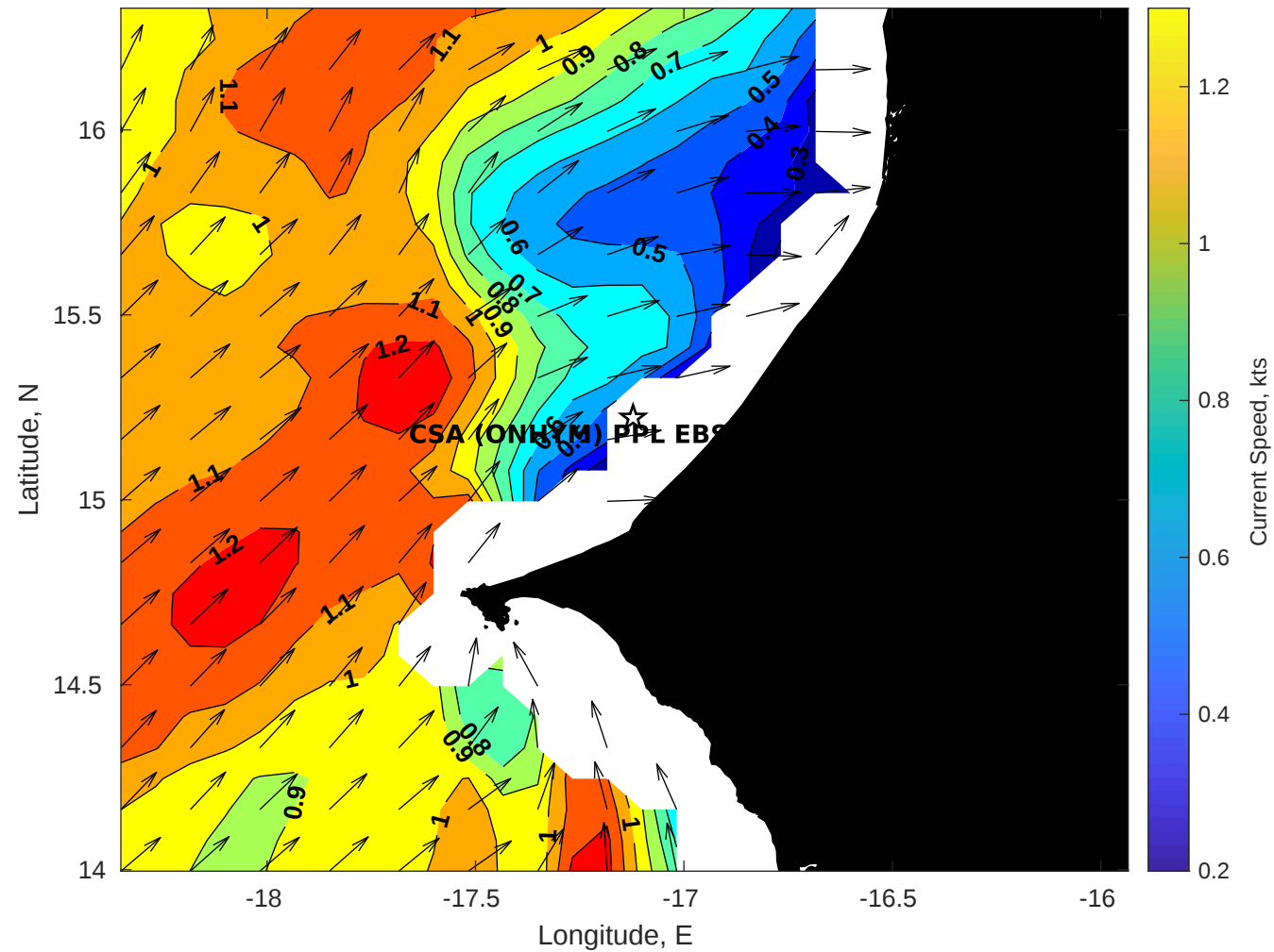
Surface Currents for CSA (ONHYM) PPL EBS - Senegal at 11-Aug-2025 00:00:00
