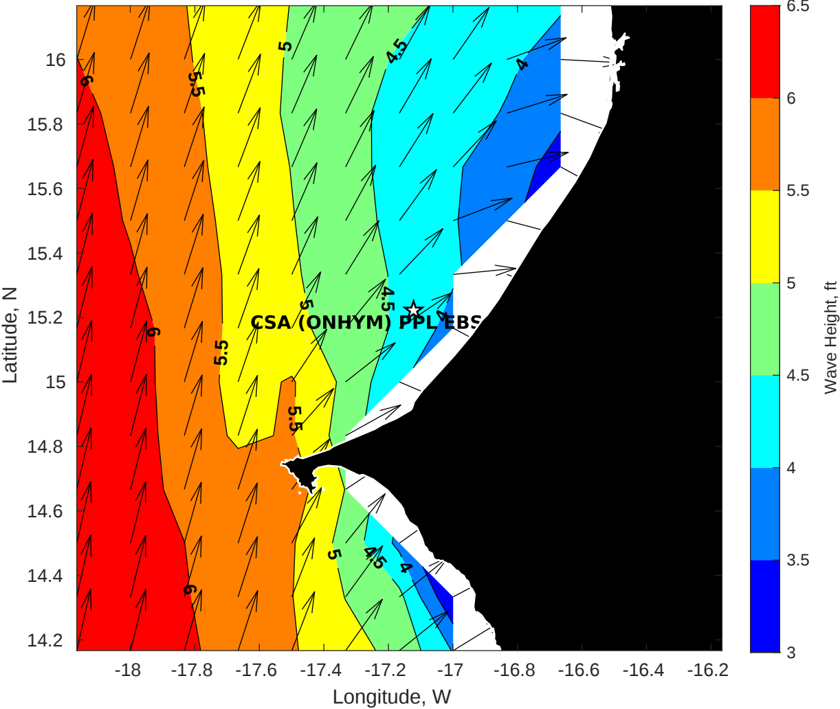
Wave Height (ft) for CSA (ONHYM) PPL EBS - Senegal at 12-Aug-2025 09:00:00
