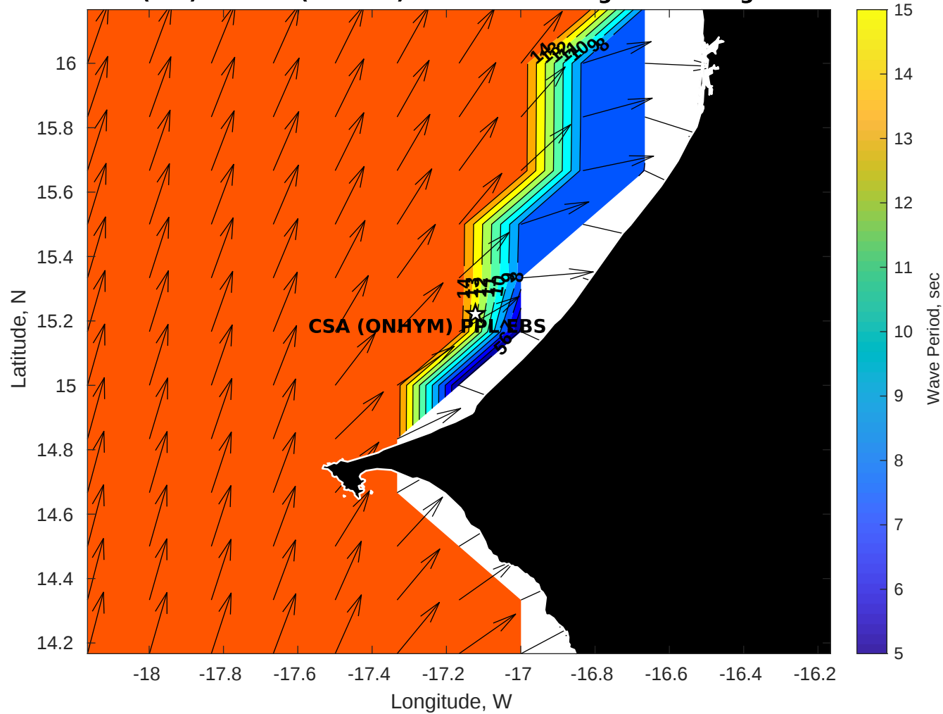
Wave Period (sec) for CSA (ONHYM) PPL EBS - Senegal at 12-Aug-2025 09:00:00
