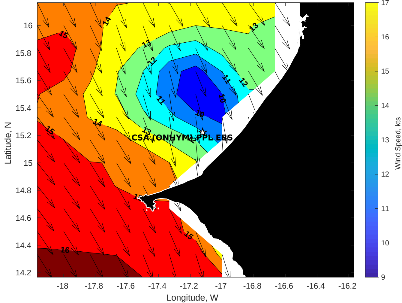
Winds (kts) for CSA (ONHYM) PPL EBS - Senegal at 12-Aug-2025 09:00:00
