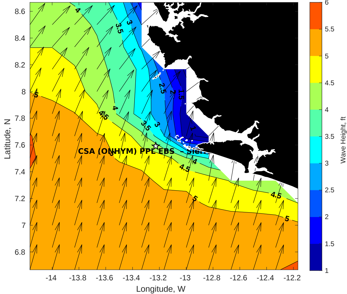
Wave Height (ft) for CSA (ONHYM) PPL EBS - Sierra Leone at 12-Aug-2025 09:00:00
