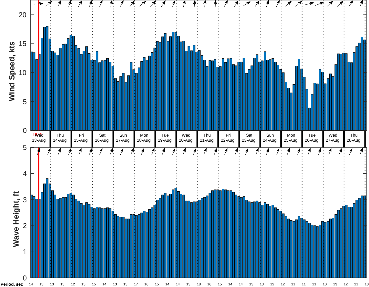
Wind & Wave Forecast for CSA (ONHYM) PPL EBS - Sierra Leone from 12-Aug-2025 01:00:00 to 28-Aug-2025 01:00:00
